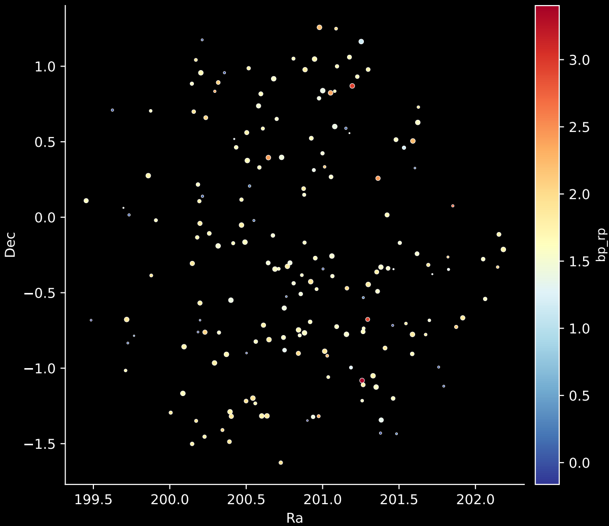
APOGEE DR17 Field: [COROTA] Stars: 187
