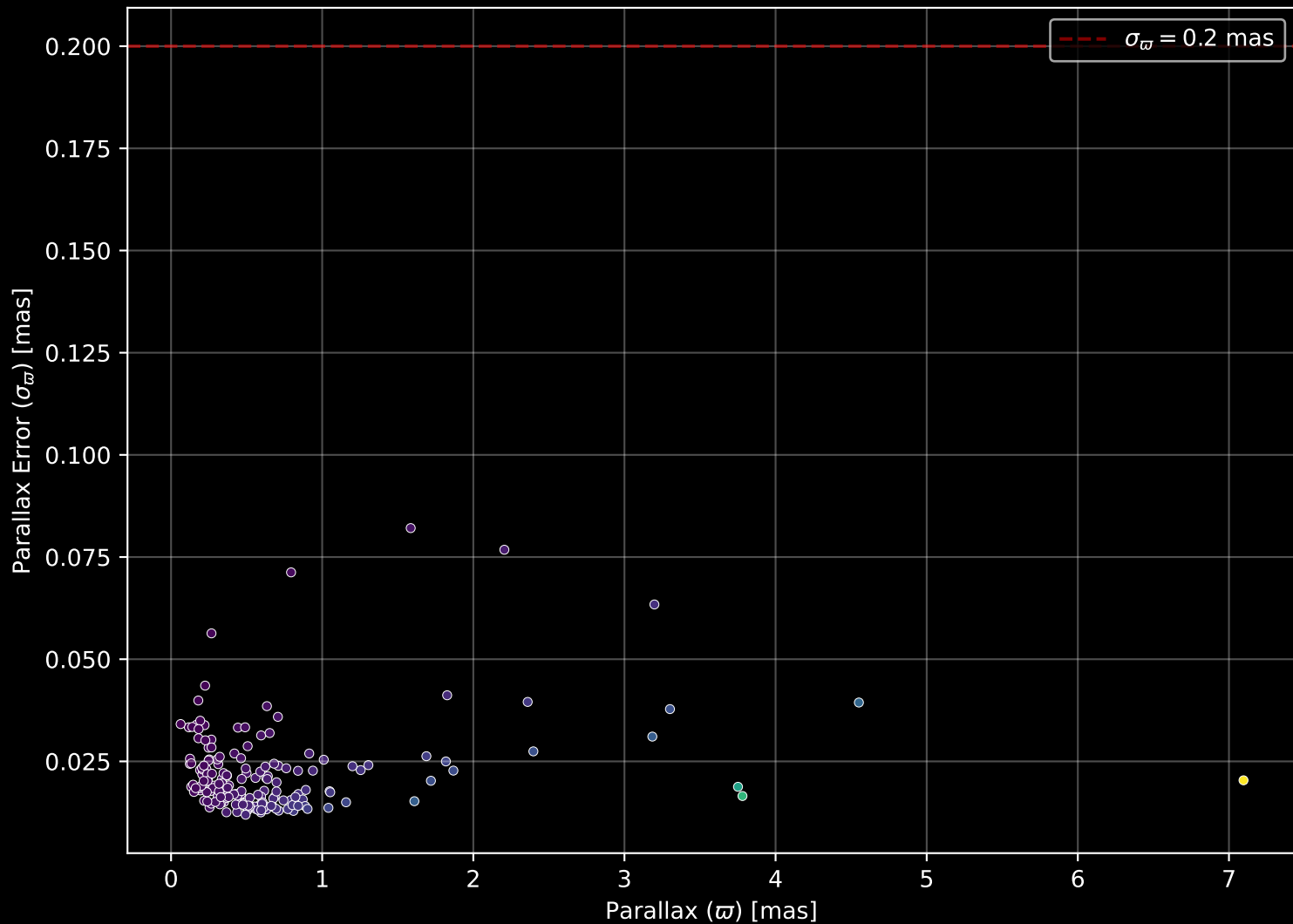
APOGEE DR17 Field: [COROTA] Parallax Quality (n= 187)
