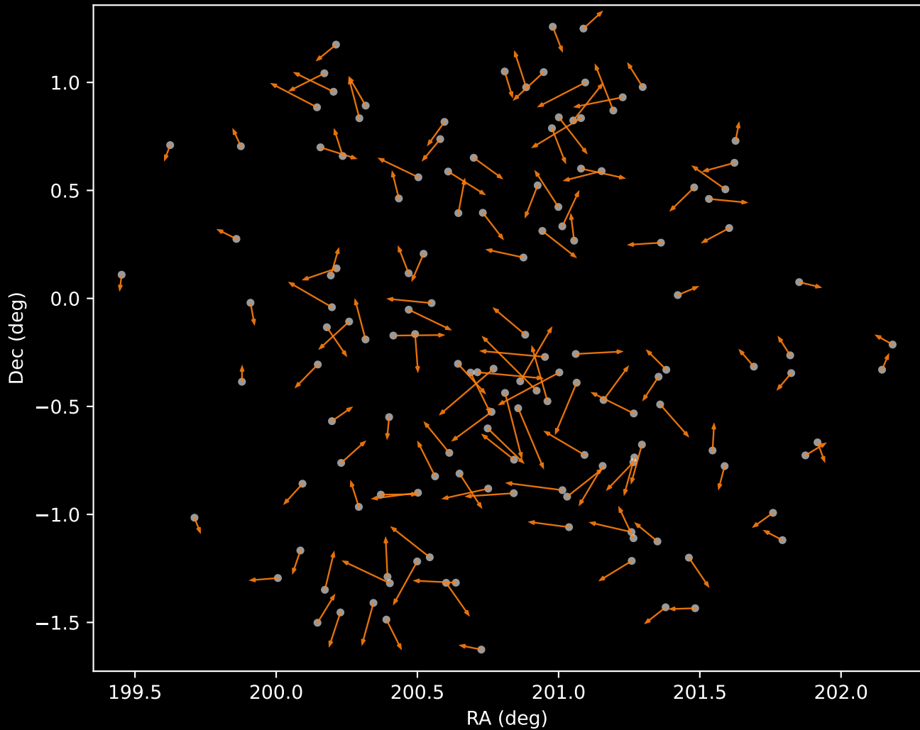
APOGEE DR17 Cluster 2 Proper Motion Vectors (n=140)
