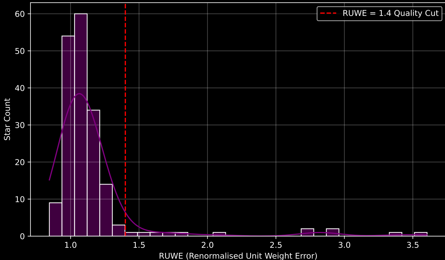
GAPOGEE DR17 Field [COROTA] RUWE Distribution (n= 186)
