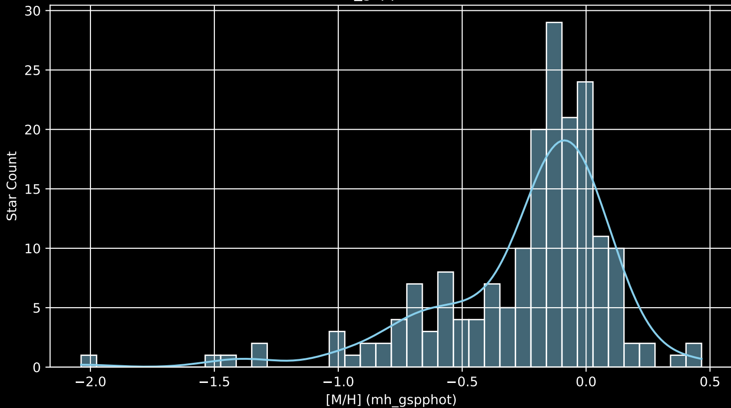
APOGEE DR17 Field: [COROTA [M/H] (mh_gspphot) (n= 187)
