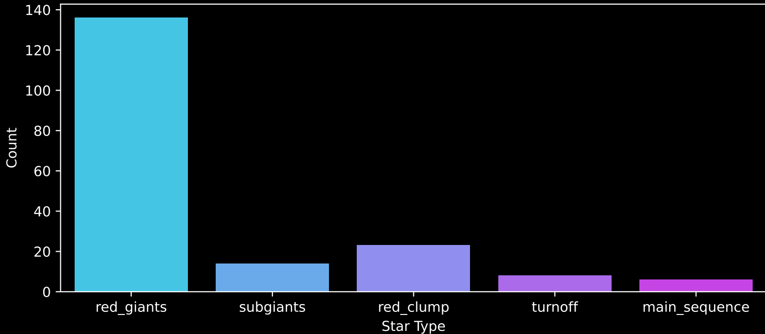
APOGEE DR17 Field: [COROTA] Count plot of Star Type
