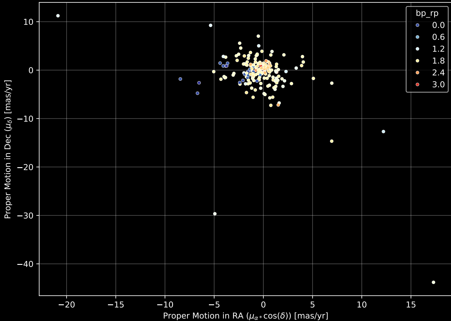
APOGEE DR17 Field: [COROTA] Proper Motion Diagram (n= 187)
