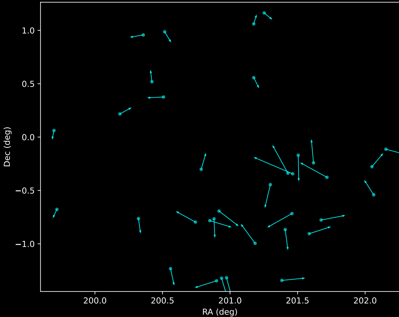
APOGEE DR17 Noise Stream Proper Motion Vectors (n=35)
